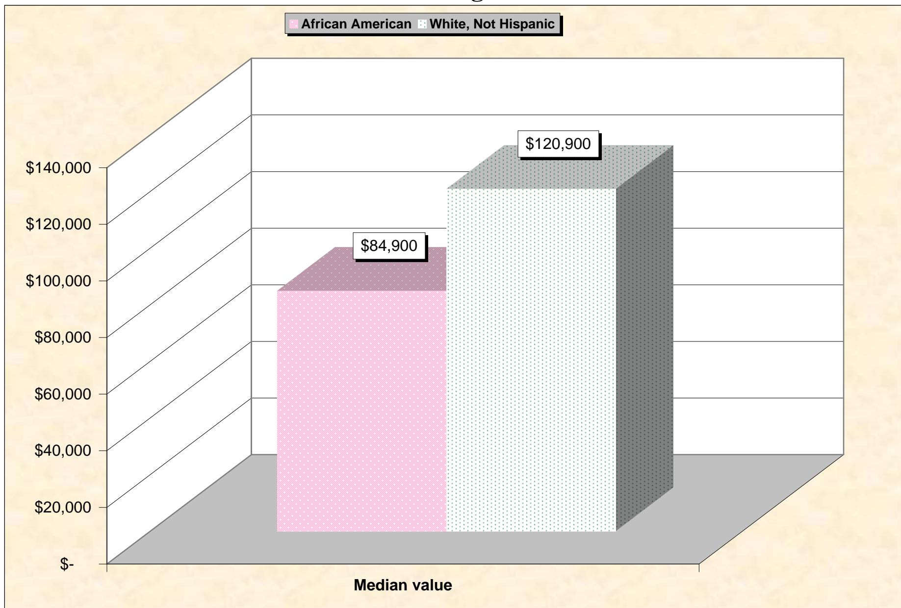
Chart 18 -- Median Home Value By Household Georgia
