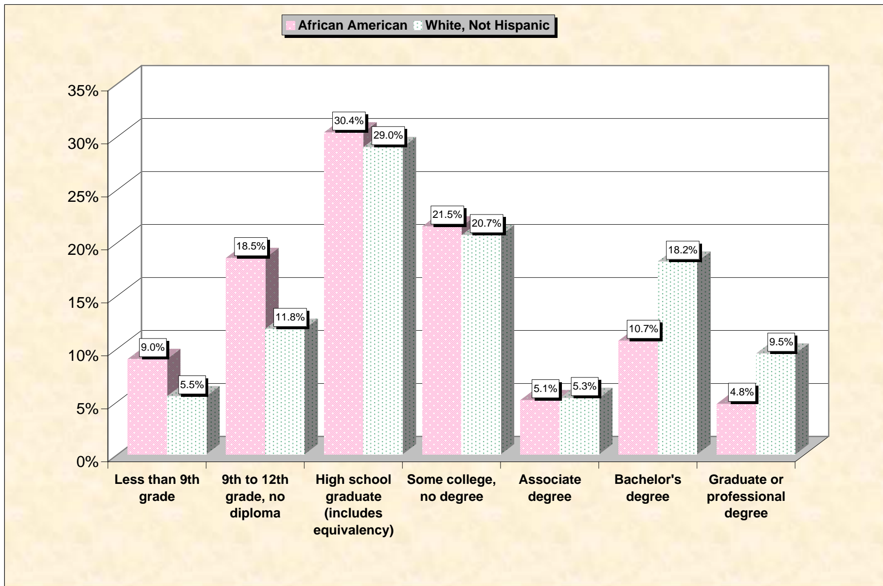
Chart 3 -- Educational Attainment (25 years and over) Georgia
