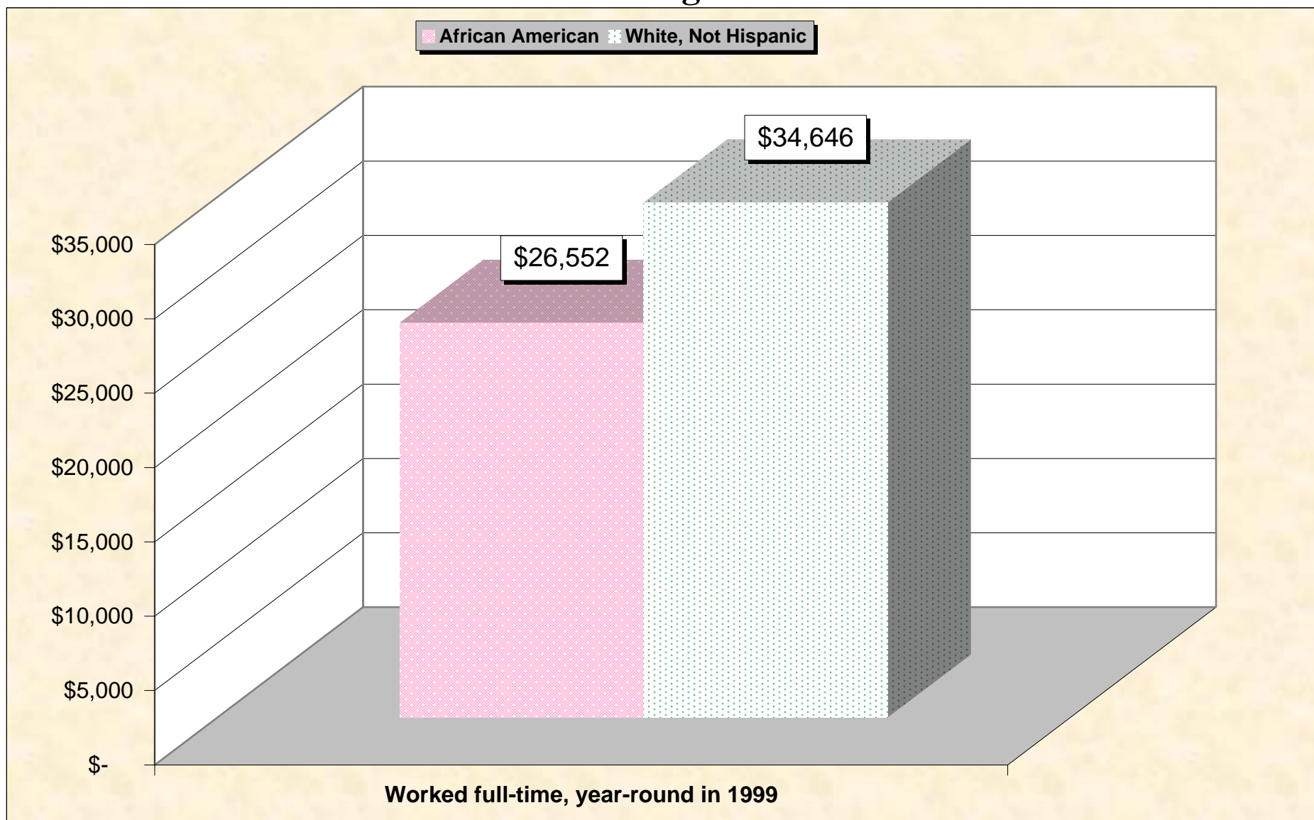
Chart 10 -- Median Earnings in 1999 Georgia
