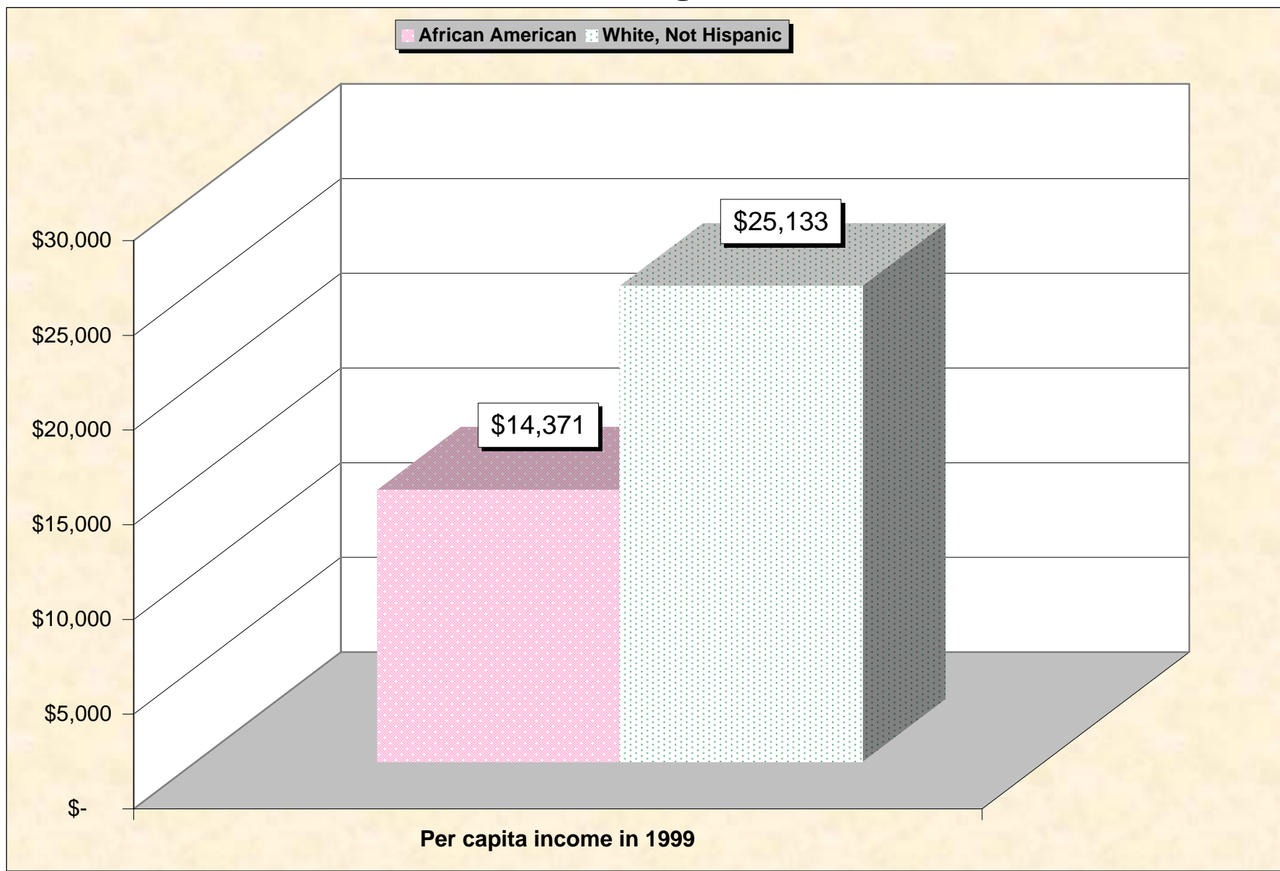
Chart 8 -- Per Capita Income In 1999 Georgia
