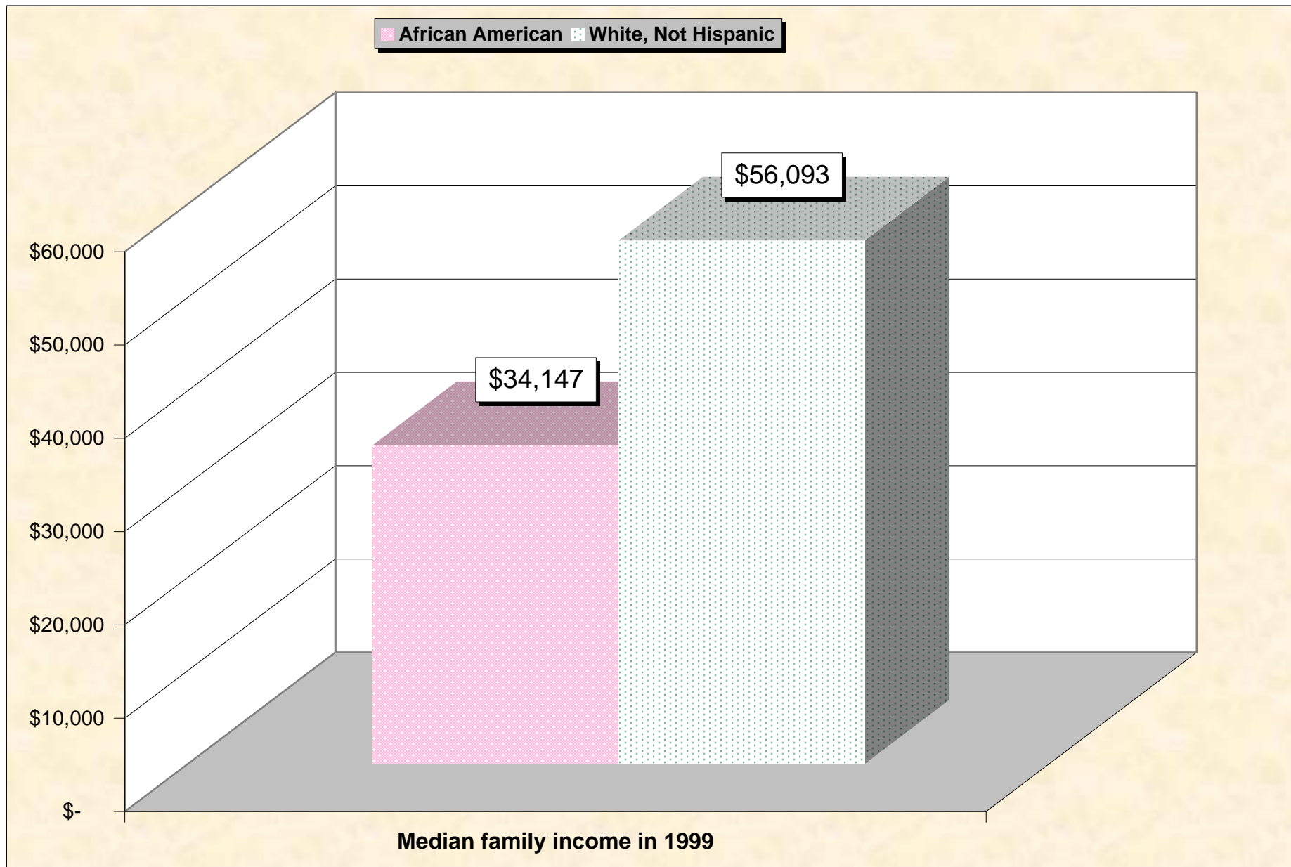
Chart 7 -- Median Family Income In 1999 Georgia
