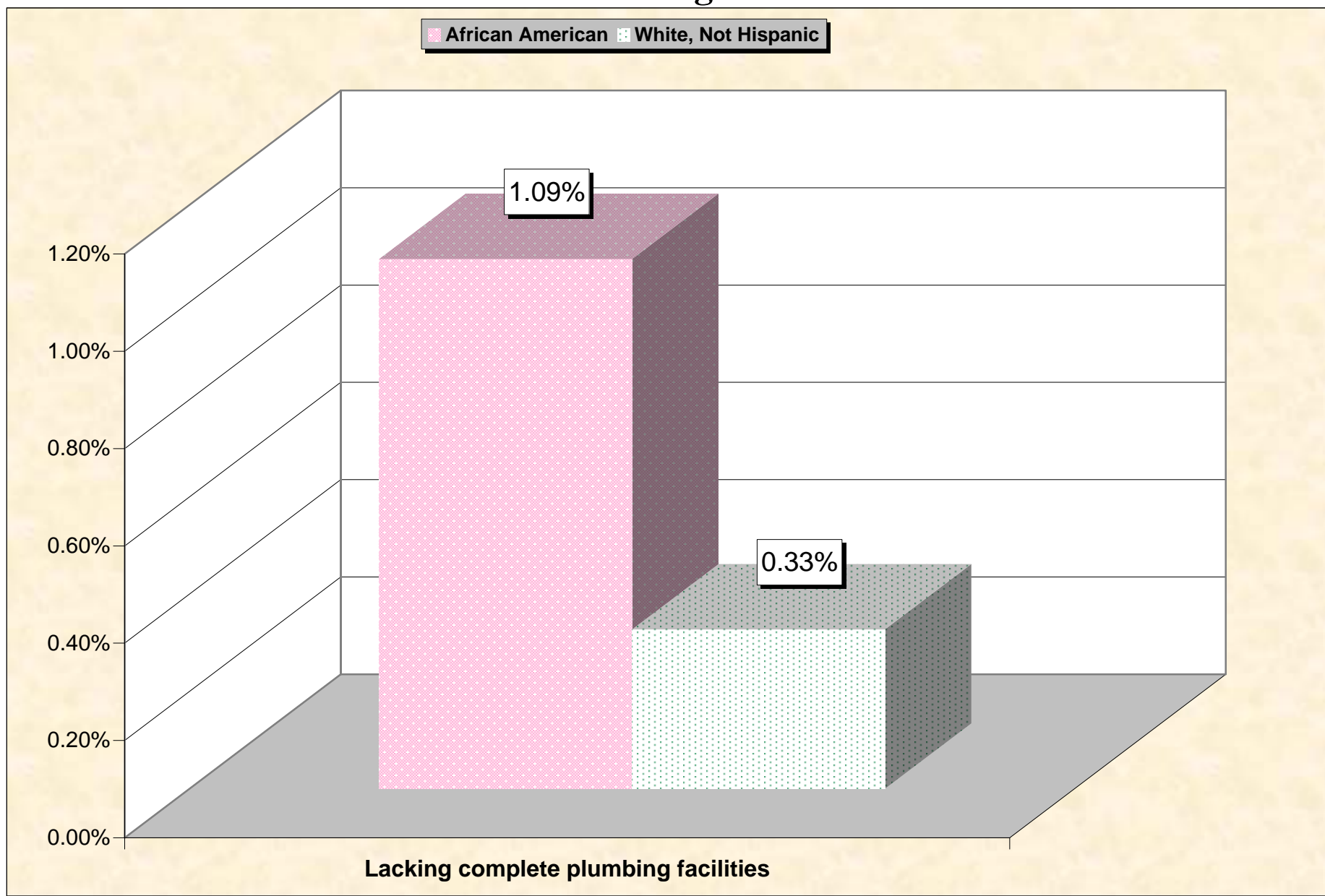
Chart 15 -- Lack of Plumbing By Household Georgia
