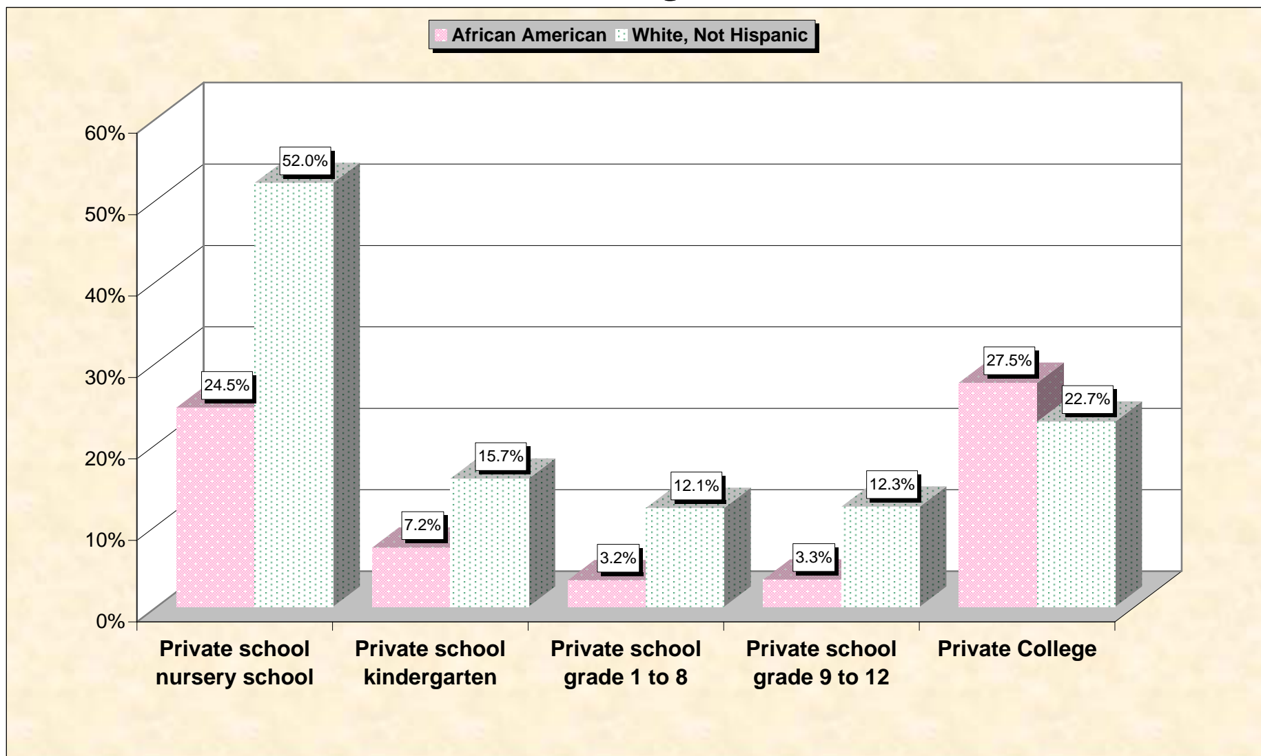
Chart 2 -- Private School Enrollment (3 years and over) Georgia
