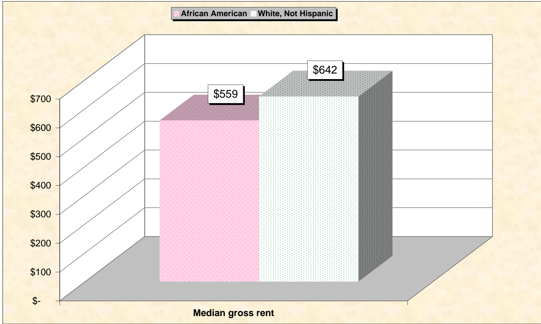
Chart 17 -- Median Gross Rent By Household Georgia
