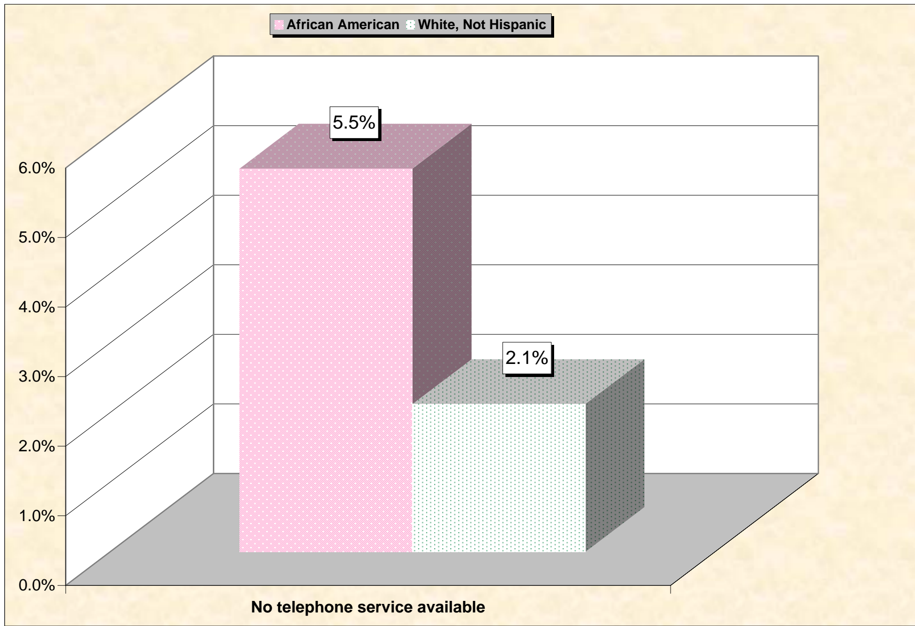
Chart 13 -- Lack of Telephone Service by Household Georgia
