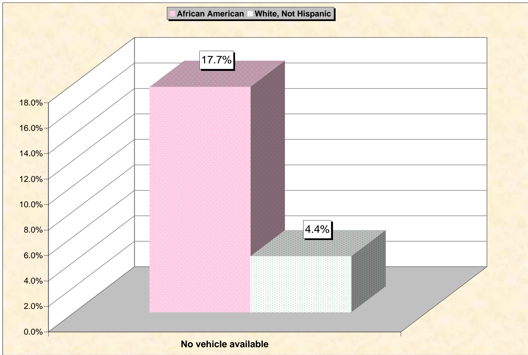
Chart 14 -- Lack of Vehicle By Household Georgia
