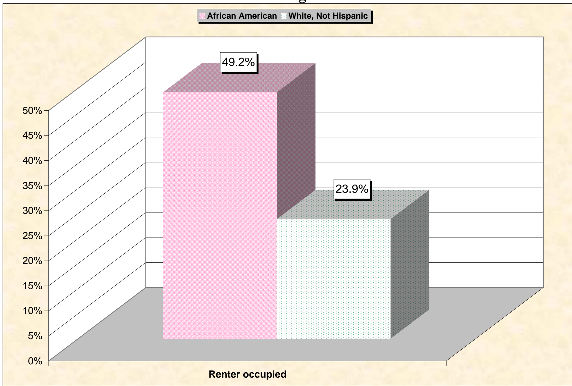
Chart 11 -- Renter-Occupied Housing Georgia
