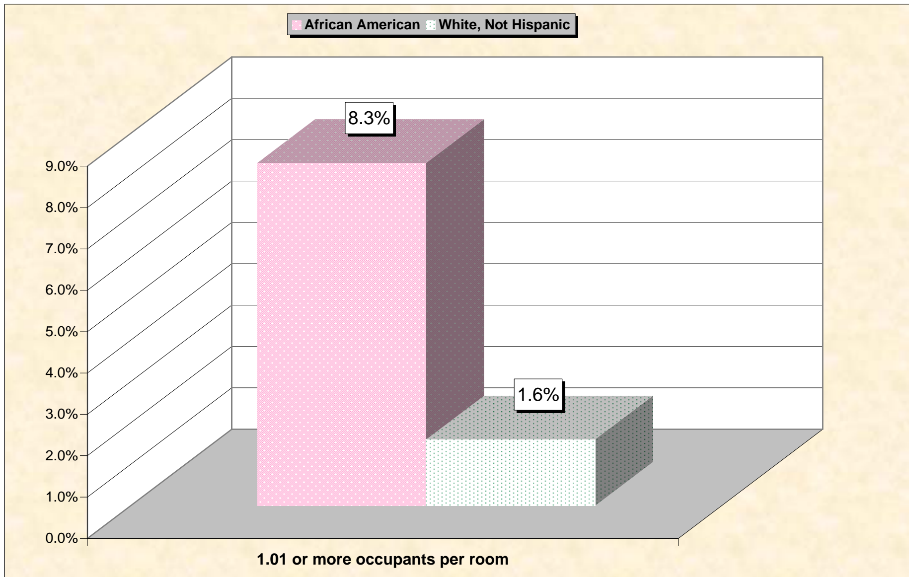
Chart 12 -- Occupants Per Room (Crowding) by Household Georgia
