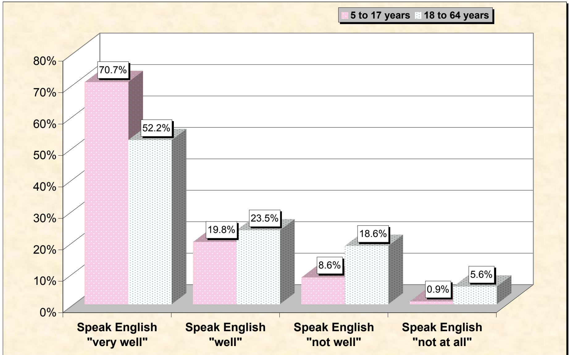
Chart 1 -- English Proficiency by Age for Persons who Speak Spanish at Home Anderson County, Texas
